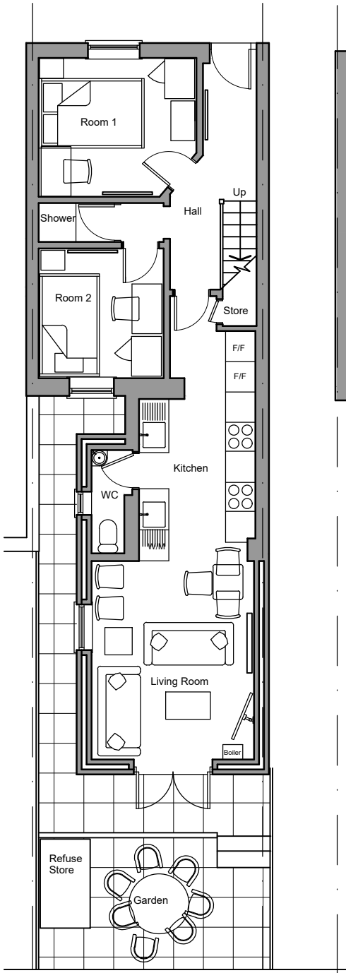
Ground Floor
